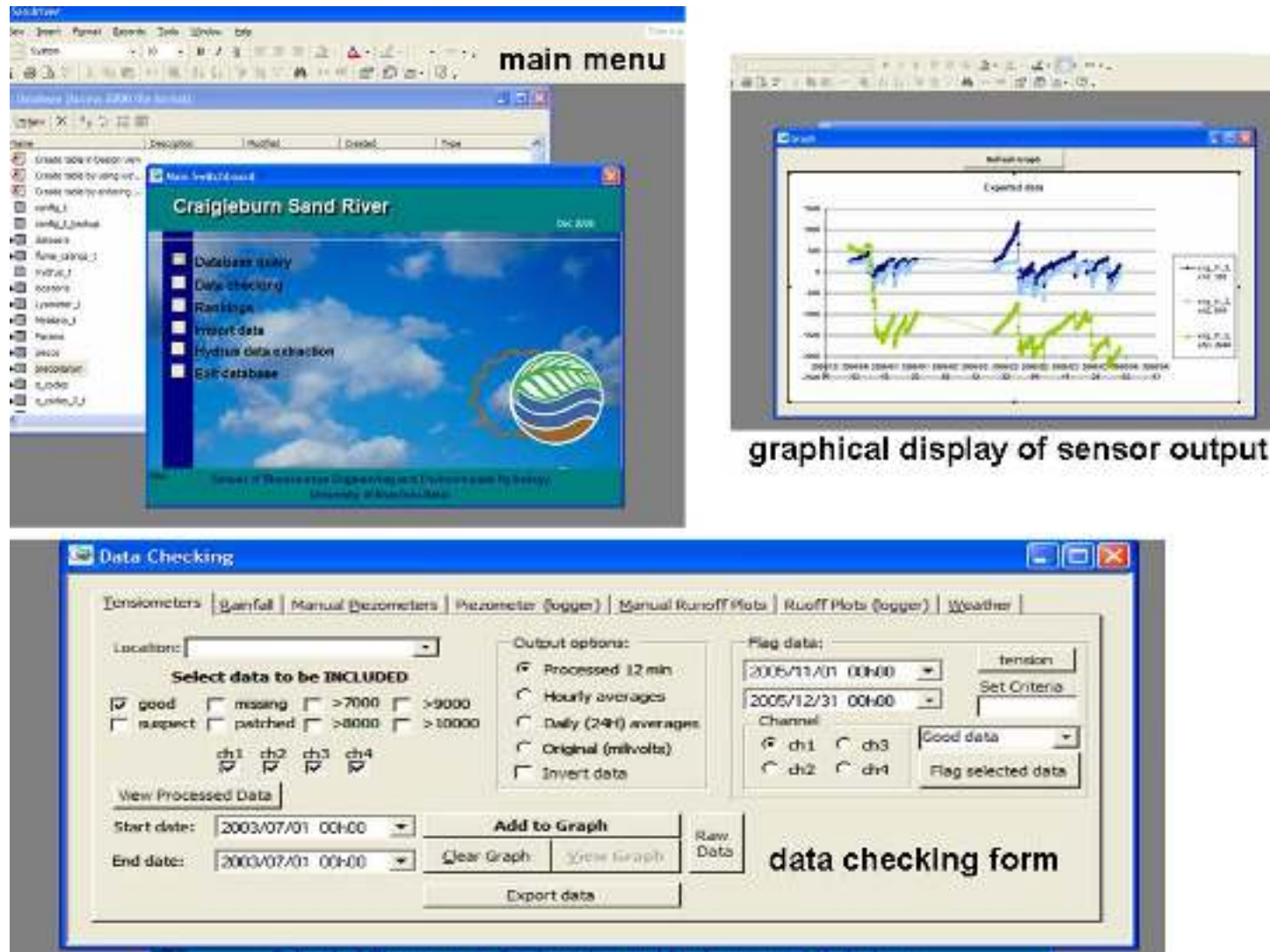
Figure 3.14: Microsoft Access Database configured for hydrometric analysis and data collection (Lorentz et al. , 2004).
