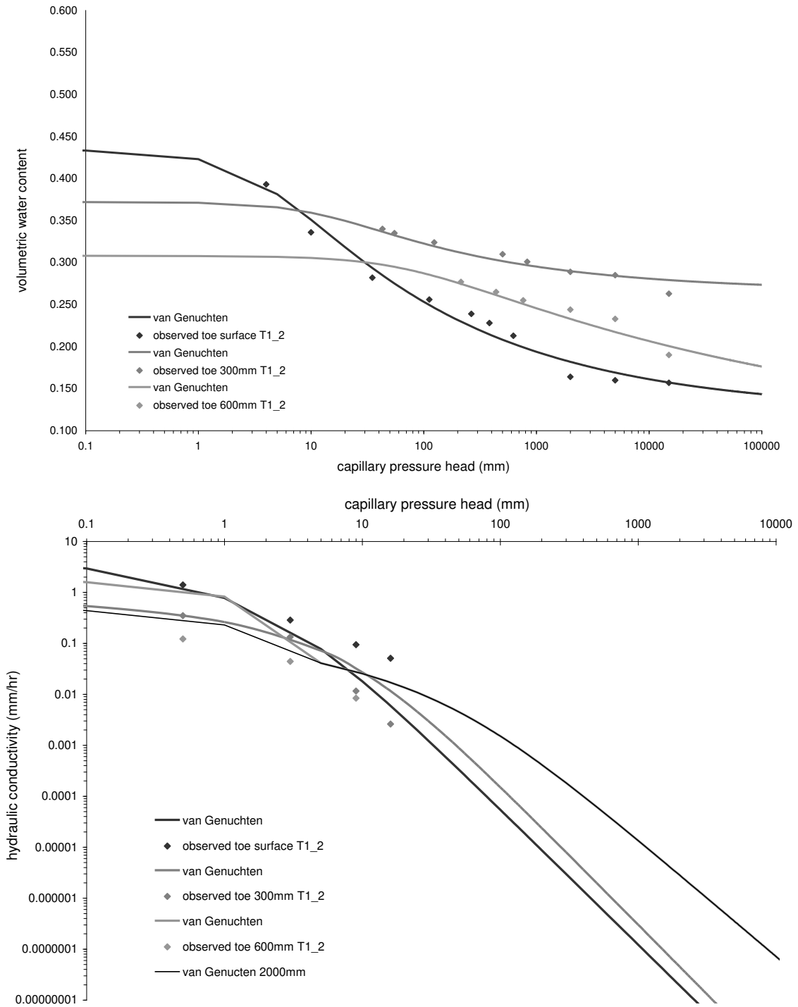
Figure iii.b: Water retention characteristics (above) and hydraulic conductivity characteristics (below) for site T1_2 used in Chapter 4 (NB double curvature close to saturation for 600 mm and 2000 mm invoking dual porosity of Vogel & Cislerova, 1988).
