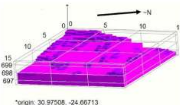
Fig. 14. Pseudo 3-D IP section of the wetland-footslope interface with chargeability values filtered to between 0–1 ms. Scales are in metres diverging from a geographical origin, vertical scale is altitude a.s.l.
