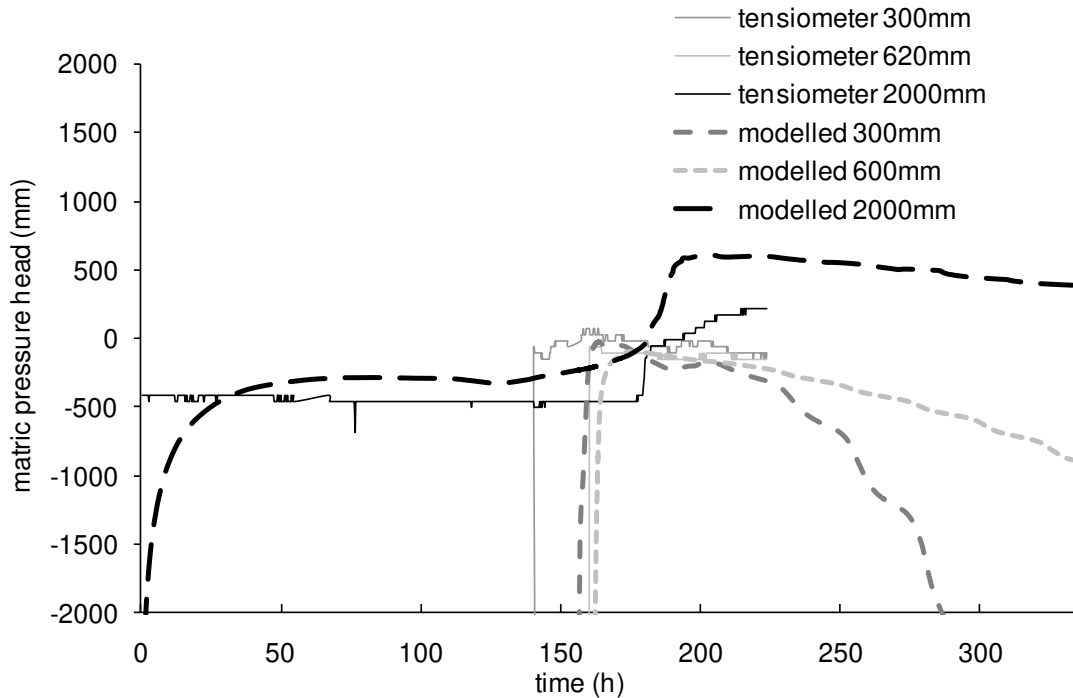
Figure 6.8e: Comparison of observed and modelled responses at and T1_3 with reduced matric pressure head range.
