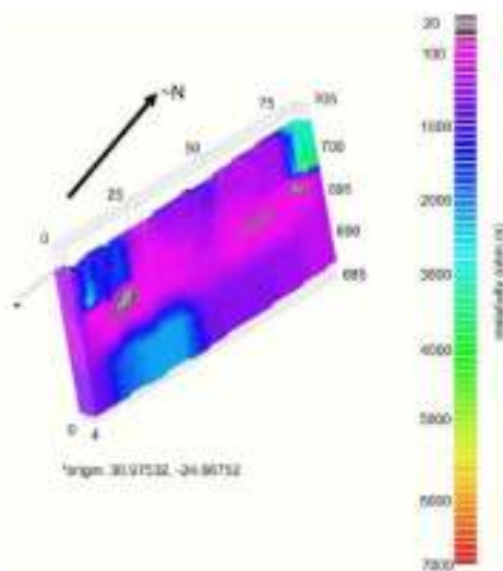
Fig. 10. Pseudo 3-D resistivity section of the SE–NW parallel transects. Scales are in metres diverging from a geographical origin, vertical scale is altitude a.s.l. (Wenner long, 2 m spacing, 8th iteration, RMS error 6.36%).
