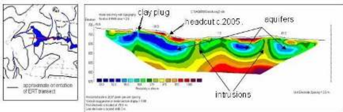
Figure 5.8: ERT longitudinal section through the erosion gully (May 2005).
