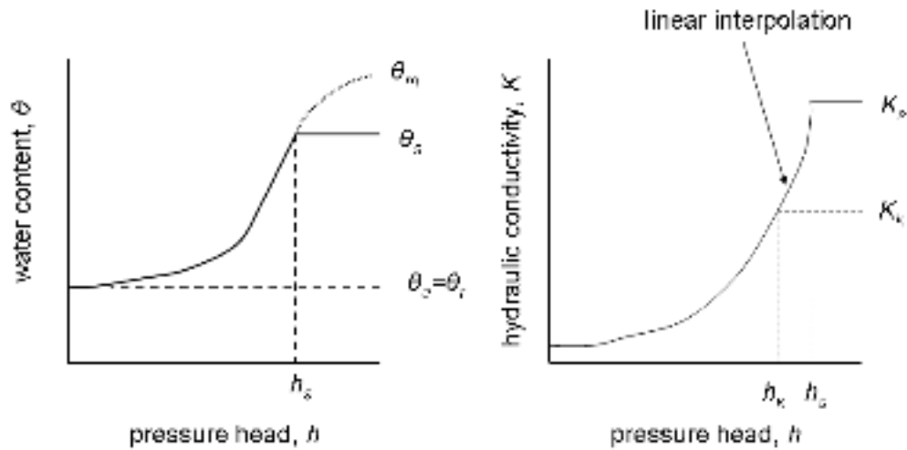
Figure 6.3: Relationship of water retention (left) and hydraulic conductivity (right) for given matric pressure heads, according the modified form of the Mualem-van Genuchten equation, by Vogel Císlerová (1988).
