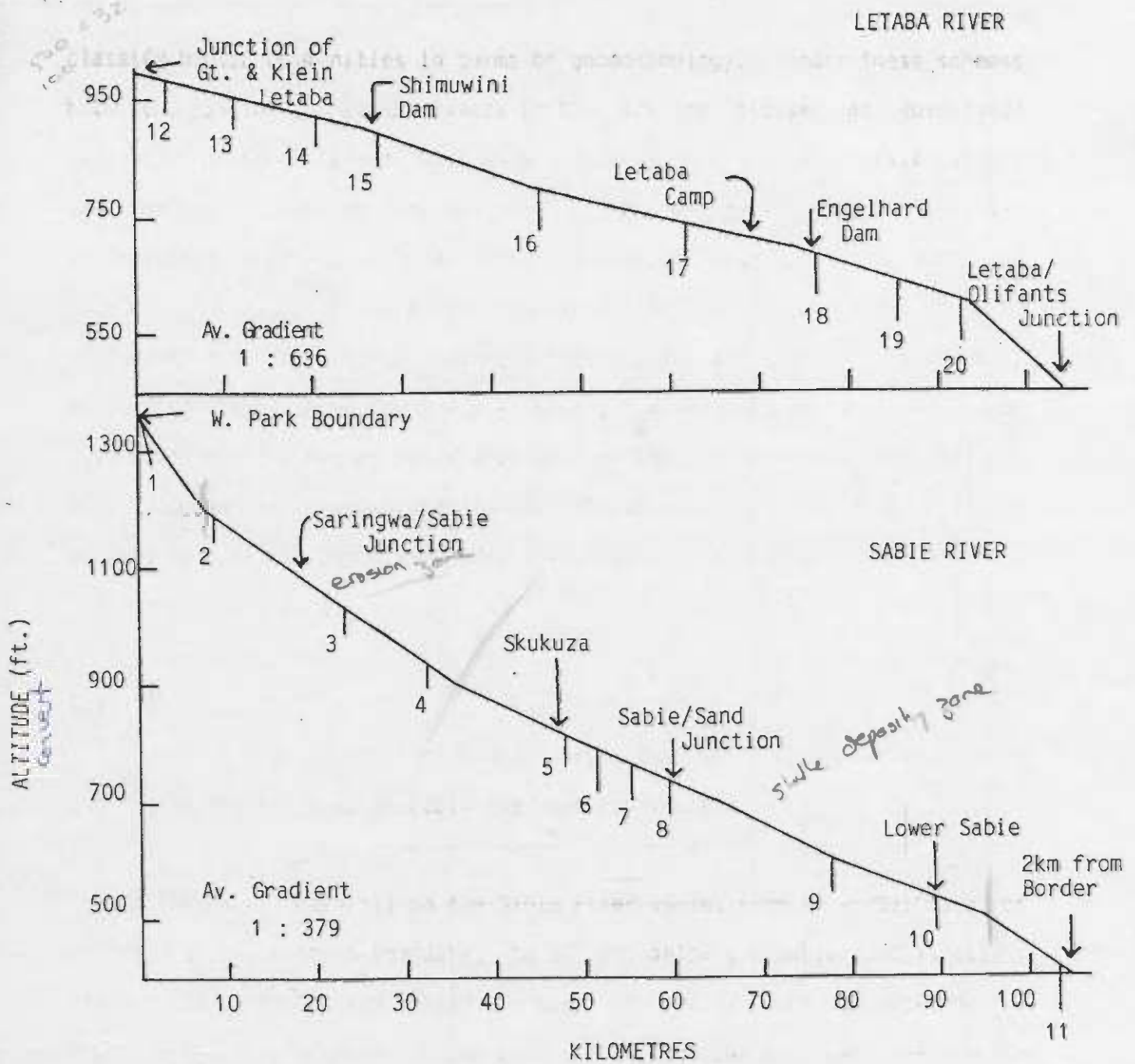
Fig. 3. Gradients of the Letaba and Sabie Rivers within the Kruger National Park. (The positions of sampling sites are marked).
